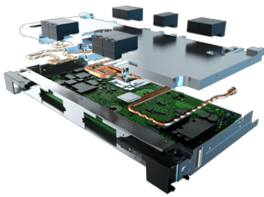
BXI L1 direct liquid cooled switch for Bull Sequana
